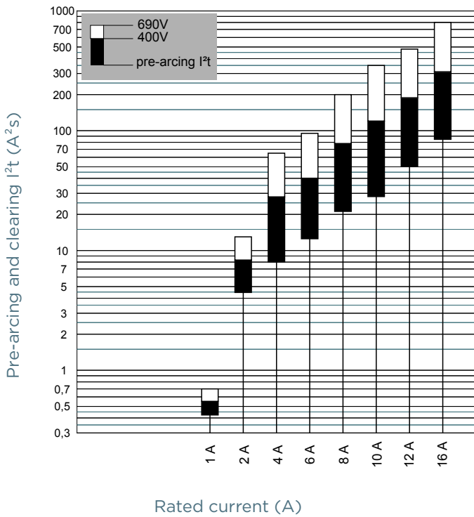
Size 10x38 690V gG without striker
