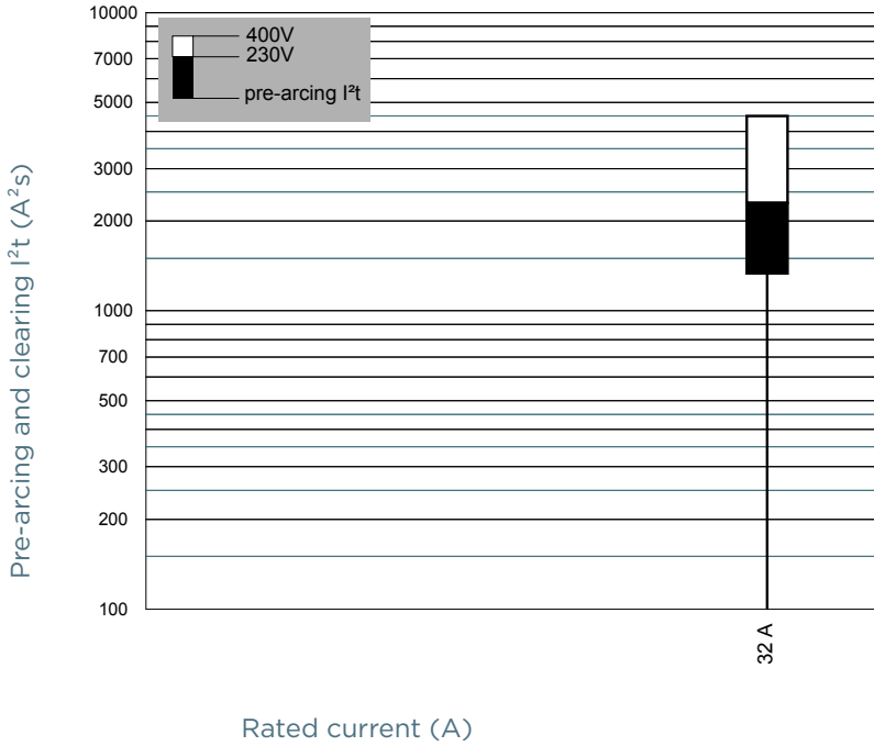
Size 10x38 690V gG without striker
